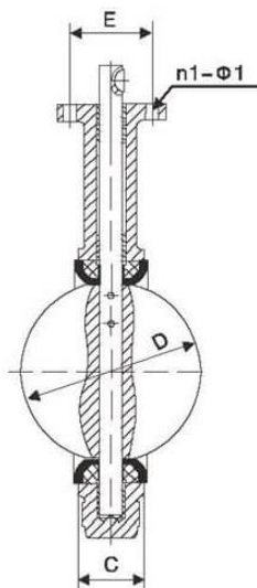
DN250(10'')~DN600(24'')
