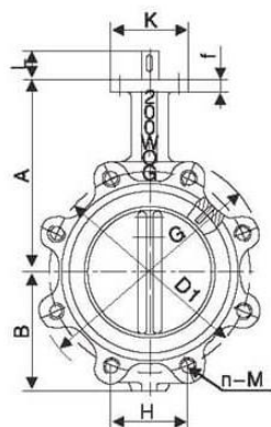
DN50(2'')~DN600(24'')
